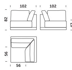
Module corner low backrest
