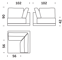
Module corner high backrest
